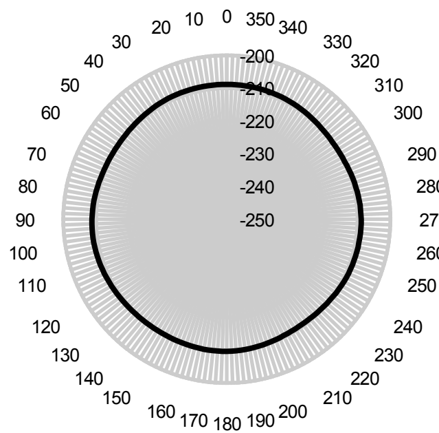
Directional Response, 20KHz XZ (Vertical)
