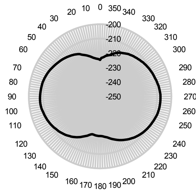
Directional Response, 100KHz XZ (Vertical)
