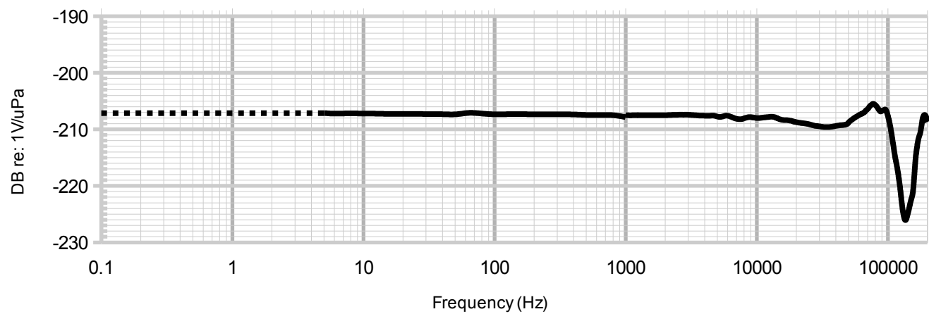
Transmitting Voltage Response
